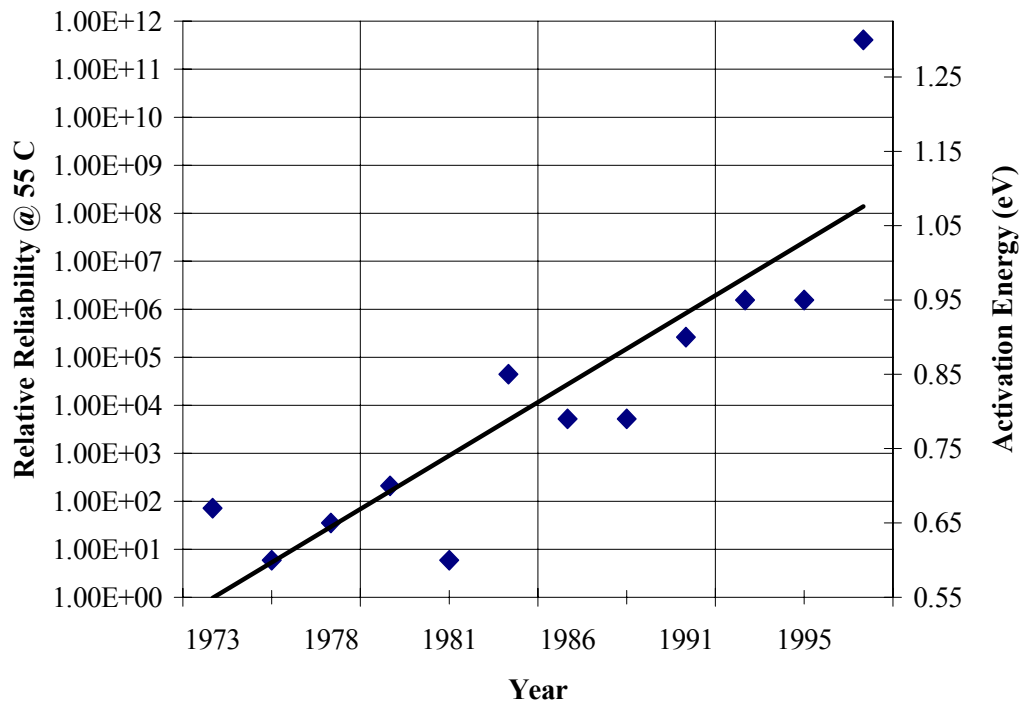
Figure 1: Pecht's Law states that semiconductor device reliability is doubling every fourteen months 2 . Reliability for this model has been measured in terms of time-to-failure. Relative reliability in the plot on a specific year is defined as the ratio of the time-to-failures at 55 °C between the specified year and 1973.
