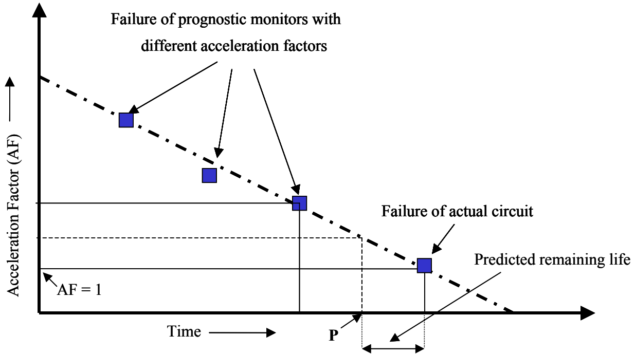
Figure 3: This picture shows a curve through the failure points of different prognostic cells mounted on the same chip as that of the actual circuit. The point with acceleration factor equals to “one” is for the failure of the actual circuit. Predicted remaining life shown in the diagram is estimated for point “P”.
