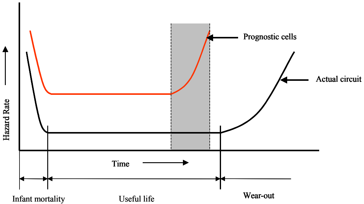
Figure 2: This shows the idealized bathtub reliability curves for the test circuit and the prognostic cell. The shaded region is the failure region of the prognostic cells, which is before the wear out region of the actual circuit.
