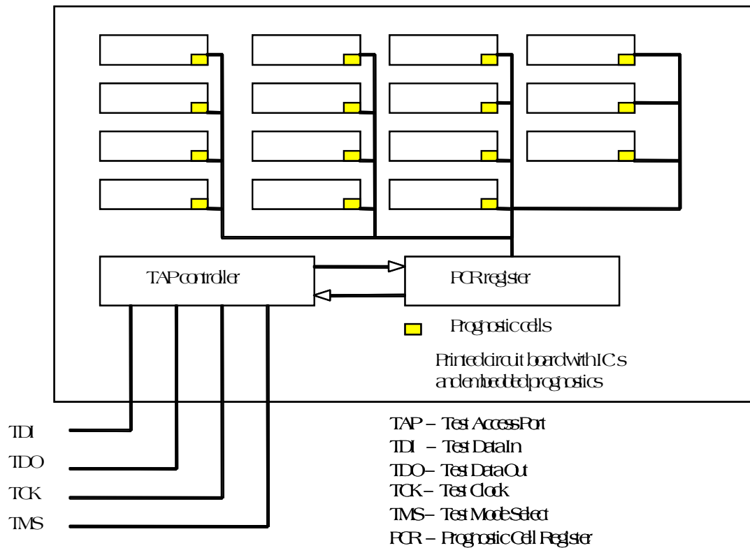
Figure 4: This schematic circuit shows the main data transfer lines in implementation of prognostic cells with JTAG data extraction.
