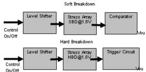
Figure 2: TDDB Block Diagram
