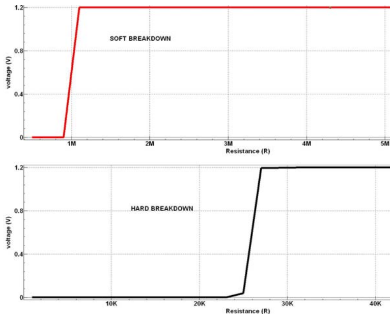
Figure 4: Simulation of TDDB Soft Breakdown and Hard Breakdown, Showing Voltage vs. Oxide Resistance
