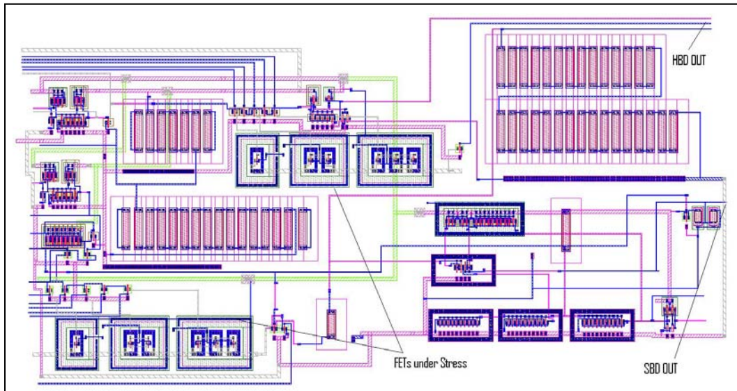
Figure 5: GDSII Layout of TDDB Cell to Detect Hard and Soft Breakdown
