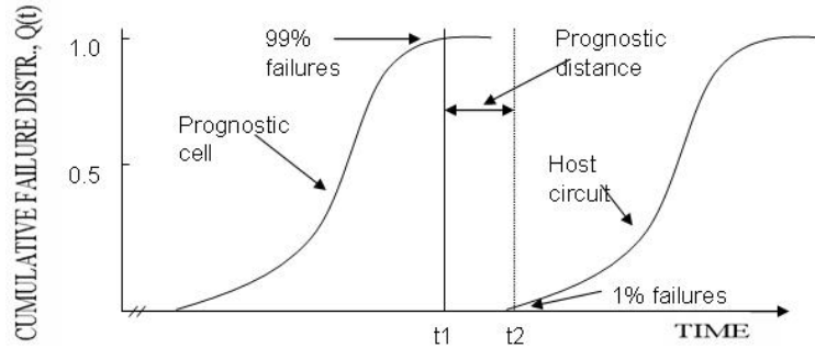
Figure 3: TDDB Cumulative Failure Distribution in Highly Accelerated Life Test (HALT)
