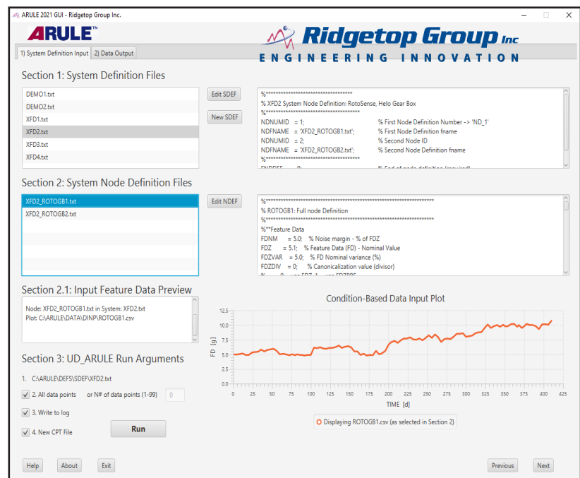
Example of condition-based gearbox data being analyzed with ARULE 2021 software program
